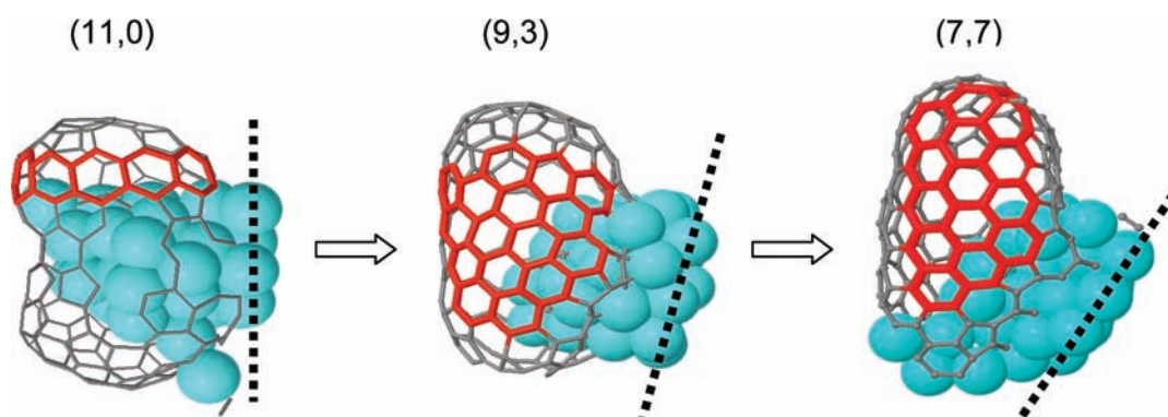
Figure 4. Evolution of chirality during the growth process. The chirality of the different structures, as defined by its diameter and chiral angle, is indicated above each structure. The dotted line indicates the surface.
